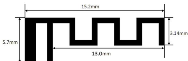
Antenna Photo & Length (mm)
